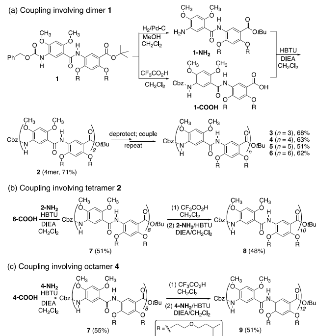
Scheme 1. Synthetic Routes of Aromatic Oligoamides
