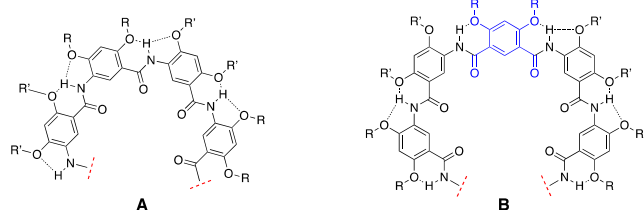
Figure 1. General structures of aromatic oligoamides having (A) an unsymmetrical (N-to-C) backbone and (B) a symmetrical backbone consisting of a central diacid residue (blue) and two identical groups. Hydrogen bonds are shown as dashed lines.
