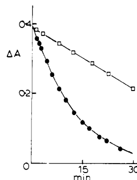
Figure 1. Plot of absorbance \Delta A changes at 487 nm (1-cm path length optical cell) for the \text{IrCl}_6^{2-} ( 1.0 \times 10^{-4} M) oxidation of \text{Mo}^{\text{IV}}_3 ( 3.7 \times 10^{-4} M) (●) and \text{Mo}^{\text{V}}_2 ( 5.9 \times 10^{-4} M) (□) at 25 °C, [\text{H}^+] = 1.00 M, and I = 2.00 M ( \text{LiClO}_4 ).
