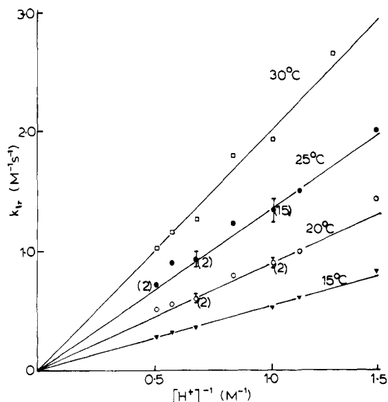
Figure 2. Dependence of second-order rate constants k_{Ir} on [H^+] for the IrCl_6^{2-} oxidation of Mo^{IV}_3 at I = 2.00 M ( LiClO_4 ). Numbers of runs averaged are indicated in parentheses.
