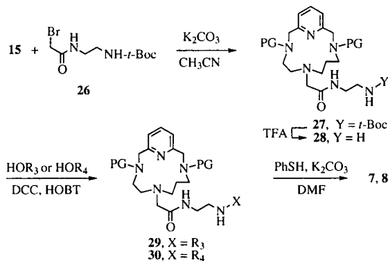
Scheme III Preparation of Compounds 7 and 8
