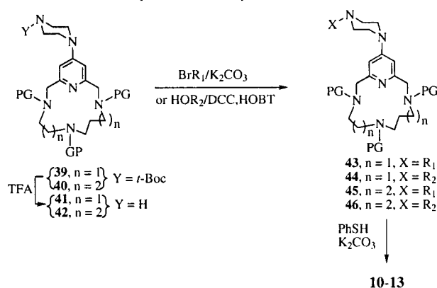
Scheme V Preparation of Compounds 10-13
