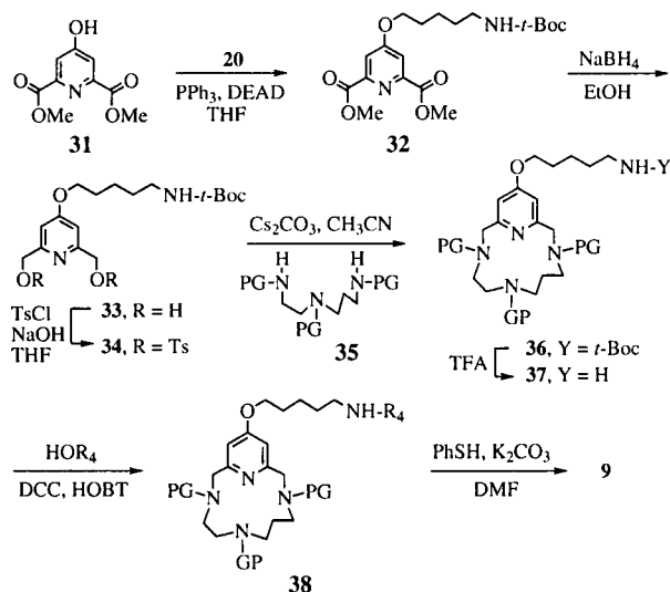
Scheme IV Preparation of Compound 9
