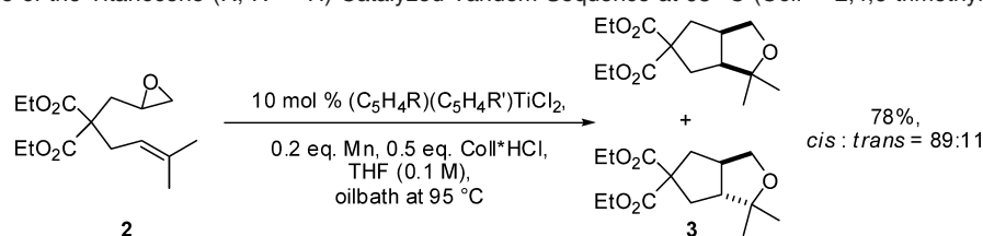
Scheme 7. Performance of the Titanocene (R, R' = H) Catalyzed Tandem Sequence at 95 °C (Coll = 2,4,6-trimethyl pyridine)
