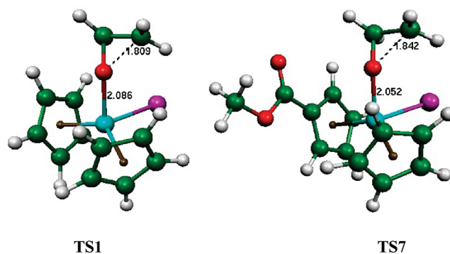
Figure 2. Transition states of oxidative addition to ethylene oxide by 1 and 7 .
