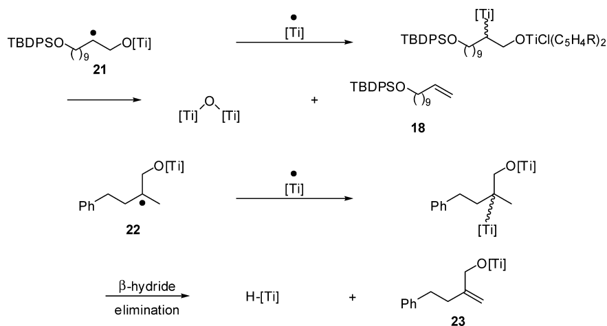
Scheme 6. Interception of \beta -Metaloxy Radicals by Titanocene(III) Reagents ( [\text{Ti}] = (\text{RC}_5\text{H}_4)(\text{R}'\text{C}_5\text{H}_4)\text{TiCl} )
