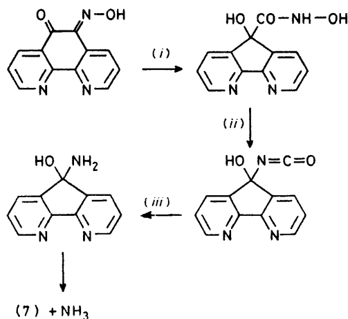
SCHEME 2 (i) OH - , benzil-benzilic acid rearrangement; (ii) OH - , Lossen rearrangement; (iii) H 2 O, -CO 2
