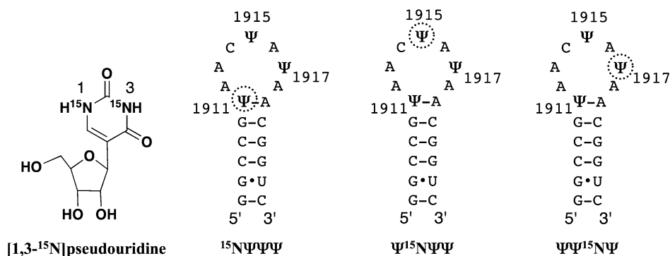
Fig. 1 The structure of pseudouridine (Ψ) and secondary structures of RNA hairpins representing H69 (positions 1906–1924) of E. coli 23S rRNA are shown. The nitrogens of Ψ are enriched with ^{15}\text{N} , and circles indicate [1,3-^{15}\text{N}]\Psi positions in the H69 hairpins.
