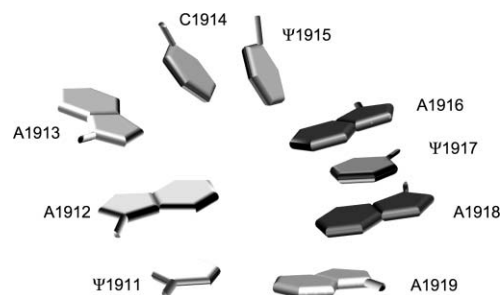
Fig. 3 A schematic representation of the H69 loop region is shown with base-stacking interactions between \text{C}_{1914} and \Psi_{1915} and \text{A}_{1916} , \Psi_{1917} , and \text{A}_{1918} , and base-pairing interactions between \Psi_{1911} and \text{A}_{1919} .
