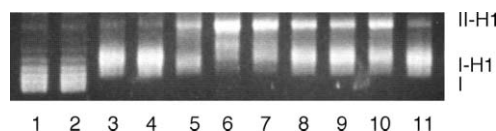
Fig. 4 Cleavage of pUC19 DNA (102 \mu\text{M} \text{bp}^{-1} DNA and 0.23 mg \text{mL}^{-1} histone H1 in 10% DMSO/10 mM Tris buffer, pH 8) by 9 . Lanes 1 and 2, DNA alone; lanes 3 and 4, DNA and histone; lanes 5–11, DNA, histone, and 9 (50, 50, 25, 13, 6.3, 3.1, and 1.5 \mu\text{M} , respectively). Mixtures in lanes 2, 4 and 6–11 were irradiated with Pyrex-filtered light from a 450 W medium pressure mercury arc lamp for 20 minutes. 22
