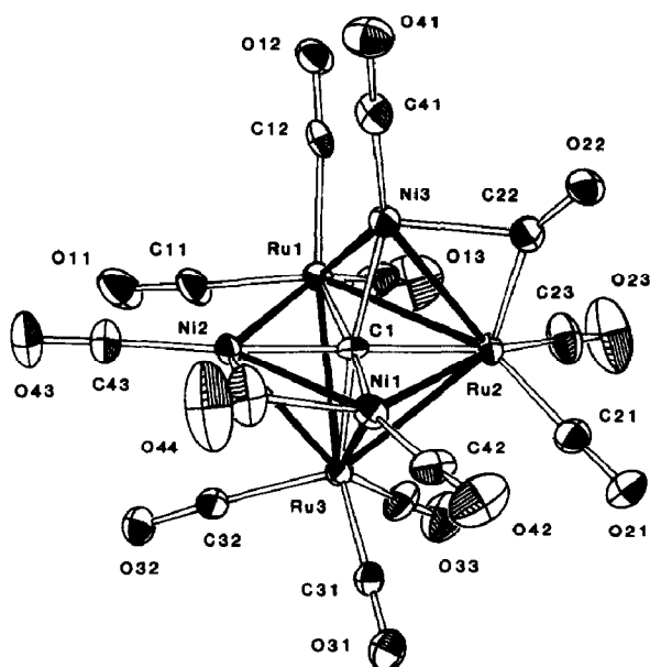
Fig. 2. ORTEF diagram for the cluster anion of [\text{PPN}]_2[\text{Ni}_3\text{Ru}_3\text{C}(\text{CO})_{13}] (VII) showing the atom labeling scheme. Thermal ellipsoids are drawn at the 35% probability level.
