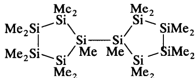
Bi(nonamethylcyclopentasilanyl) (2)
