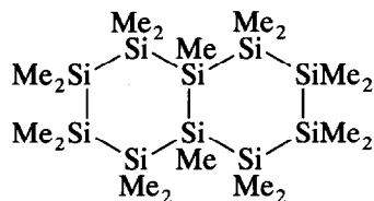
Octadecamethylbicyclo[4.4.0]decasilane (1)
