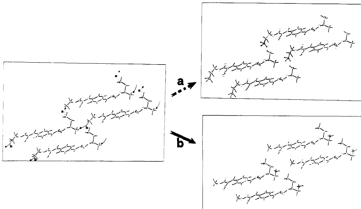
Figure 4. (Left) Contacts between the side chains of molecules located at (0,0,0), (1,2,1), and (1,1,1) in the real structure of monomer ( S )-(+)-1. (Right) Hypothetical structures obtained by transferring one methyl group between sec -butyl and ethyl moieties, following paths a or b.
