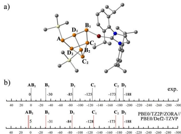
Fig. 3 (a) The proposed DFT-optimized structure of the intermediate observed in the reaction between (TMS)_3P_7 and NHC^{Dipp}CuCl . The H atoms are omitted for clarity. (b) The experimental ^{31}P\{^1H\} NMR chemical shifts observed at the 1:0.7 ratio of the reactants and the calculated chemical shifts.
