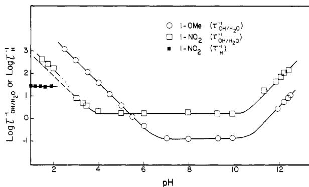
Figure 1. pH profiles for \tau_{OH/H_2O}^{-1} and \tau_H^{-1} .
