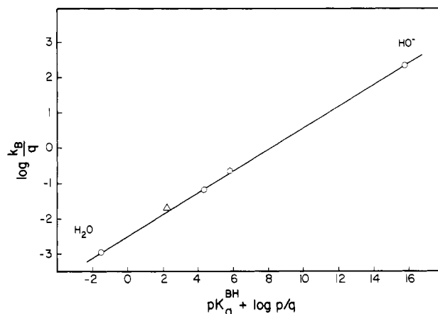
Figure 2. Brønsted plot for acetate and cacodylate ion catalyzed water addition to 1-OMe , including the water and \text{OH}^- -reactions. \Delta refers to chloroacetate ion; see Discussion.
