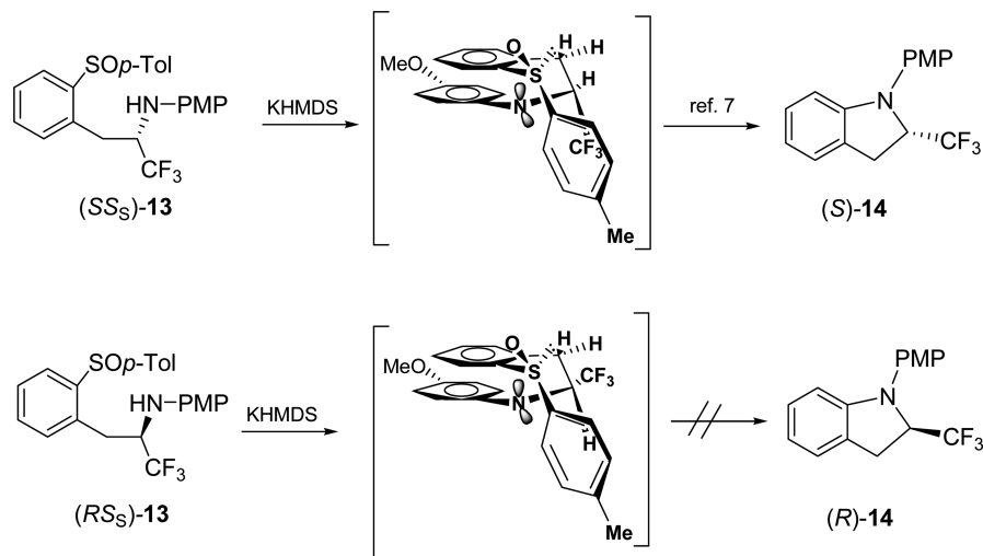
Figure 2. Evolution of (SS S )-13 and (RS S )-13 with KHMDS.
