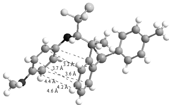
Figure 3. View of the X-ray structure of compound anti -17 showing the almost parallel geometry of the rings A and B and the interatomic distances of some significant nuclei.
