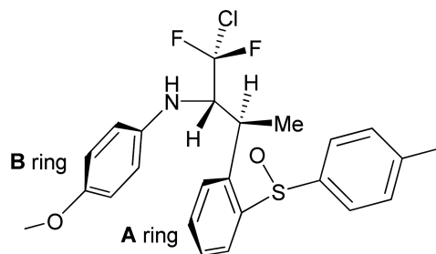
Figure 3. View of the X-ray structure of compound anti -17 showing the almost parallel geometry of the rings A and B and the interatomic distances of some significant nuclei.
