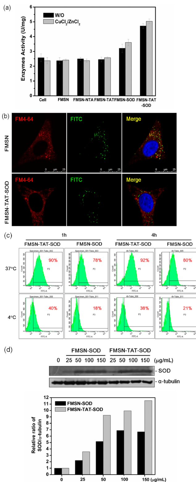
Figure 4. Effect of the TAT, \text{Cu}^{2+} , \text{Zn}^{2+} , and temperature on the delivery activity of SOD. HeLa cells were first pretreated with FMSN-TAT-SOD and control FMSN for 4 h. (a) Metal effect on the activity of FMSN-TAT-SOD. Copper ion (0.05 mM) and zinc ion (0.05 mM) were added into the culture medium and incubated for 24 h before FMSN-TAT-SOD and control FMSN treatment. The specific activity of SOD was determined by pyrogallol method. (b) Confocal microscopy analysis of MSN in endosome. The living unfixed cells were cotreated with endosome-specific marker FM 4–64 (5 \mu\text{g/mL} ) and analyzed by confocal microscopy for an endosomal colocalization
