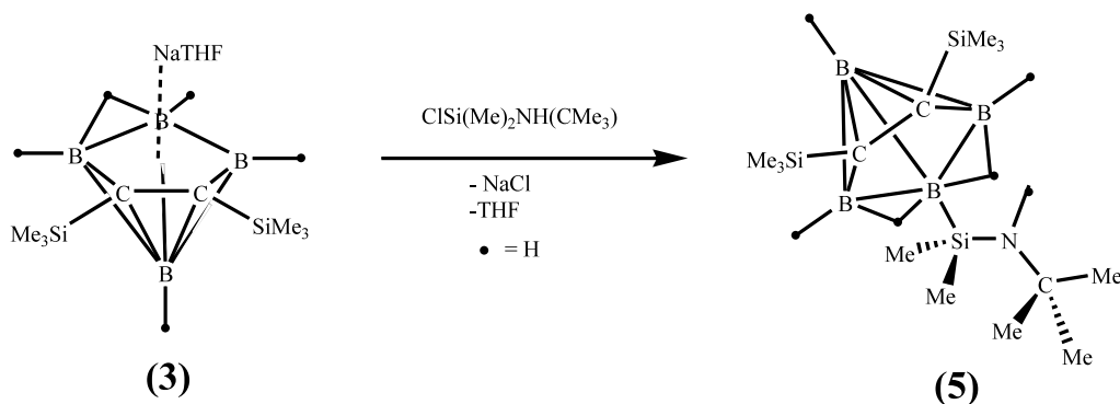
Scheme 1. Synthesis of 5 .
