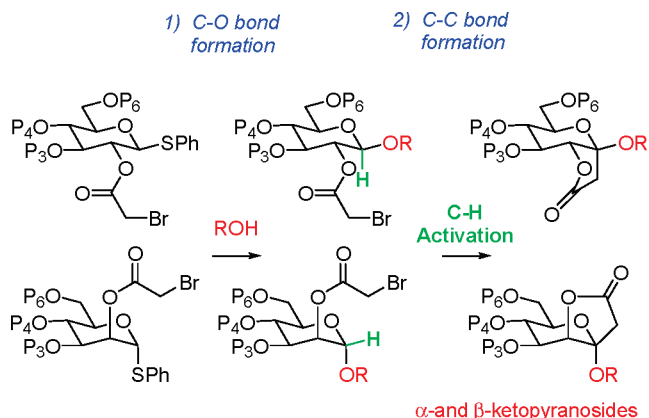
Scheme 2. Carbene-Mediated Synthesis of Ketopyranosides
