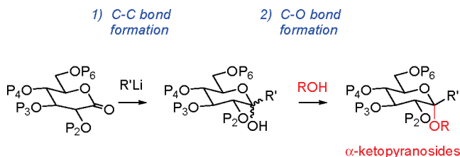
Scheme 1. Synthesis of Ketopyranosides from \delta -Lactones
