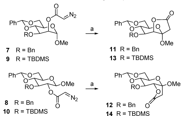
Scheme 4. Influence of 3- O -Protecting Groups a
