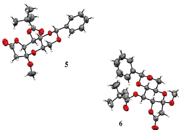
Chart 1. ORTEP Representations of 5 and 6
