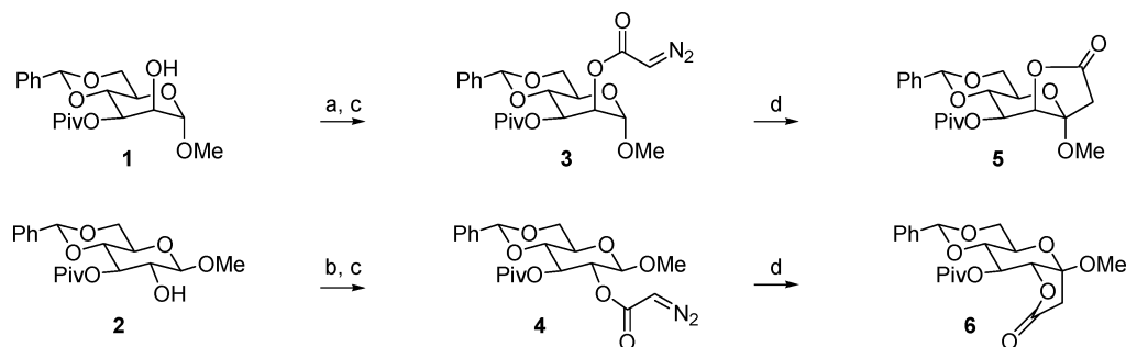
Scheme 3. Carbene-Mediated Activation of the Anomeric C–H Bond on Model Compounds a
