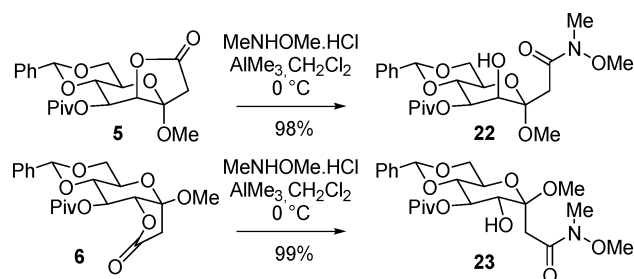
Scheme 7. Ring-Opening of γ-Lactones 5 and 6
