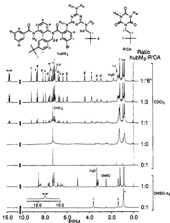
Figure 1. Spectra of the 1 H NMR titration of hubM 3 (500 MHz, 10 mM in CDCl 3 ) with R'CA. The peak assignments are shown at the top of the figure. The bottom two spectra show hubM 3 and R'CA alone in DMSO- d 6 for reference.
