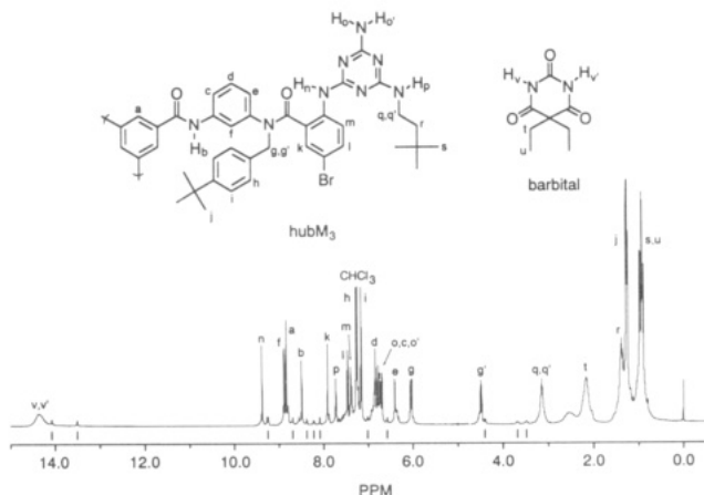
Figure 8. ^1\text{H} NMR spectrum of \text{hubM}_3(\text{barbital})_3 (500 MHz, \text{CDCl}_3 ). The major resonances in the spectrum correspond to the \text{C}_3 symmetrical isomers and are assigned. The minor resonances, some of which are indicated with lines above the scale ( \sim 5\% of the material), may correspond to the unsymmetrical isomers. These resonances are not caused by impurities in the sample.
