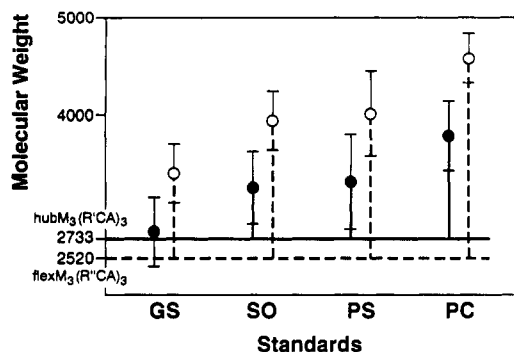
Figure 6. Experimental molecular weights of \text{hubM}_3(\text{R}'\text{CA})_3 (●) and \text{flexM}_3(\text{R}''\text{CA})_3 (○) determined by vapor pressure osmometry using four different molecular weight standards. The solid and dashed horizontal lines correspond to the calculated MWs of \text{hubM}_3(\text{R}'\text{CA})_3 and \text{flexM}_3(\text{R}''\text{CA})_3 , respectively. The four MW standards were GS = N,N -bis-( t -Boc)gramicidin S (MW 1342), SO = sucrose octaacetate (MW 679), PS = polystyrene (average MW 5050, polydispersity = 1.05), and PC = perbenzoyl \beta -cyclodextrin (MW 3321). The error bars correspond to the sum of the standard deviations of the VPO measurements of the standard and unknown. These experiments were performed at 37 °C in \text{CHCl}_3 over the concentration range 2–16 mM of complex.
