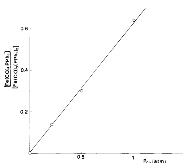
Figure 1. [Fe(CO)_4PPh_3]/[Fe(CO)_3(PPh_3)_2] vs. P_{CO} plot for the reaction between [Fe(CO)_4(H)SiPh_3] and PPh_3 at 25 °C in toluene ( [PPh_3] = 5 \times 10^{-2}\text{ M} ), [Fe(CO)_4(H)SiPh_3] = 6 \times 10^{-3}\text{ M} ). The concentration ratio was obtained by measuring the absorbance ratio of the CO stretching bands of the mono- and disubstituted complexes. 3
