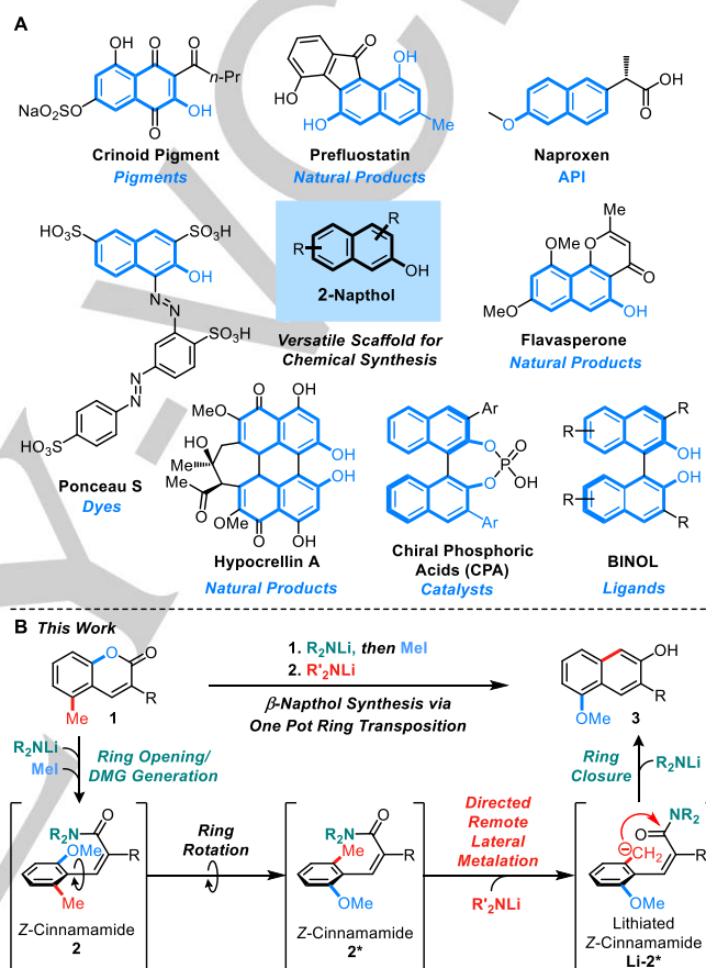
Figure 1. A) 2-Naphthols in natural and bioactive molecules, drugs, and materials. B) Synthesis of 2-naphthols 3 from coumarins 1 employing a one-pot ring transposition.
