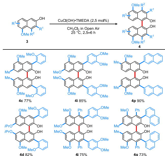
Scheme 3. Highly substituted BINOL Derivatives 4 from 2-Naphthols 3 .
