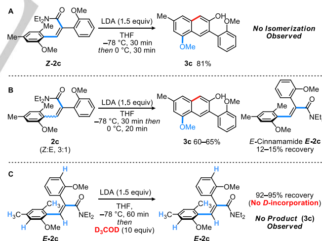
Scheme 2. Mechanism of the remote lateral metalation reaction of cinnamamide 2c .
