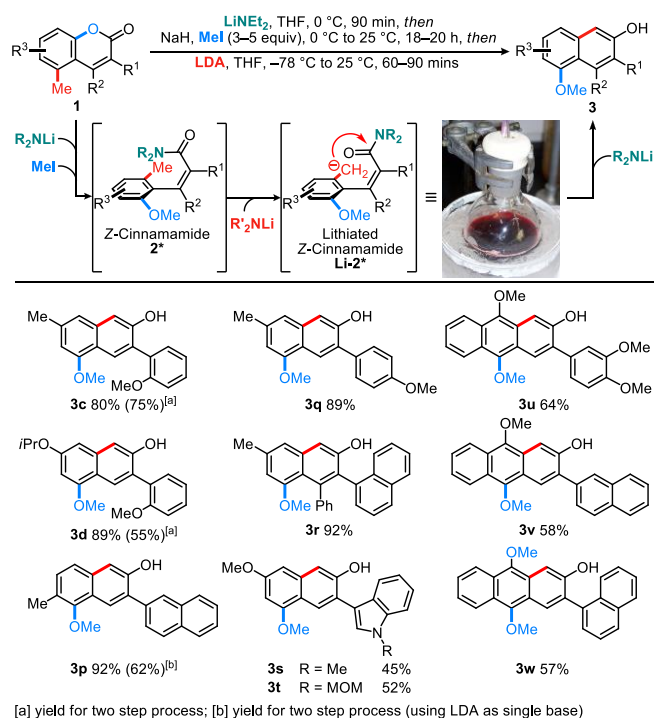
Scheme 1. One-pot synthesis of 3-aryl-2-naphthols 3 from coumarins 1 .
