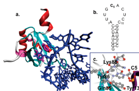
Figure 1. (a) The U1A–SL2 RNA complex from the X-ray cocrystal structure. 5f (b) SL2 RNA. (c) An expanded view of the structure.
