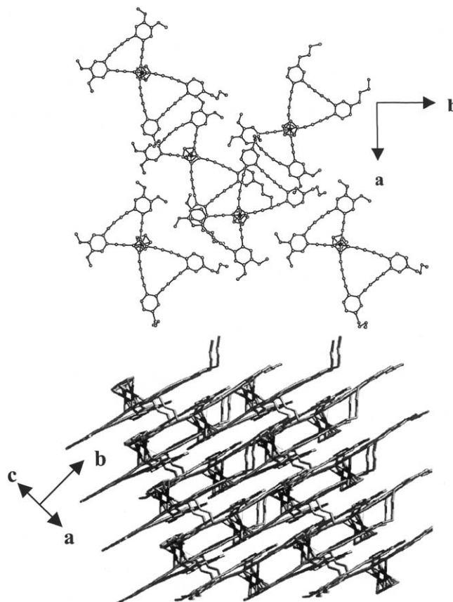
Fig. 4. Packing of the unsymmetrical butterfly 17 in the solid-state. Top, view onto the large hydrocarbon ligand. Bottom, layered structure of 17 . The layers are ca. 3.6 Å spaced apart, with the CpCo units and the butyl groups filling the interstitial interlayer spaces.
