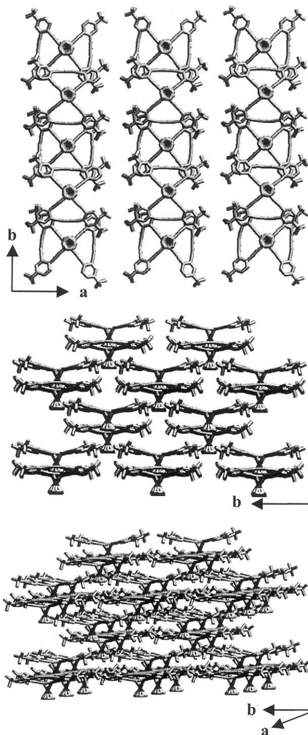
Fig. 2. Packing of the organometallic butterfly 9a . The packing pattern is such that the hydrocarbon ligands in two adjacent layers are packed in a staggered fashion. The molecules in each layer are rotated by 90° with respect to each other, which gives an overall tetragonal symmetry to this packing arrangement.
