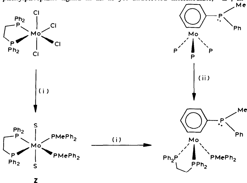
SCHEME 1. (i) 2 \text{PMePh}_2 , excess Mg, THF, 22^\circ\text{C} , 2.5 h, 75%; via a rapid rearrangement of postulated intermediate Z , S = solvent or \eta^2\text{-Ph} [1,2]; (ii) \text{PPh}_2\text{CH}_2\text{CH}_2\text{PPh}_2 , 22^\circ\text{C} , 30 min, 75% [1].
