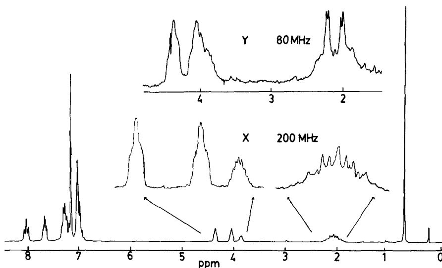
Fig. 2. The ^1\text{H} NMR spectrum at 200 MHz of \text{Mo}(\eta^6\text{-PhPPh}_2)(\text{CNBu}')(\text{DPPE}) (1h) in \text{C}_6\text{D}_6 with amplification of the region \delta 1.5–4.5 (inset X). Inset Y shows the pattern obtained at 80 MHz (see Table 2).
