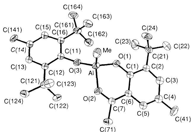
Fig. 1 The molecular structure of [\text{AlMe}(\text{dbmp})(\text{bhmap})] 1 . Thermal ellipsoids are drawn at the 30% level, and the hydrogen atoms are omitted for clarity.
