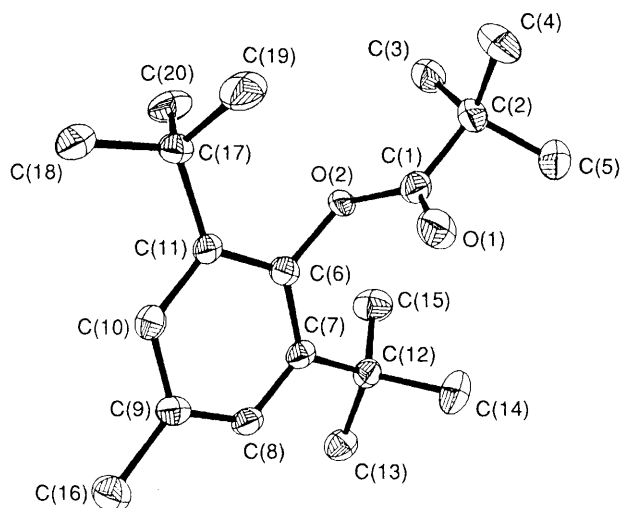
Fig. 3 The molecular structure of \text{O}=\text{C}(\text{dbmp})\text{Bu}^{\text{I}} 12 . Thermal ellipsoids are drawn at the 50% level, and the hydrogen atoms are omitted for clarity.
