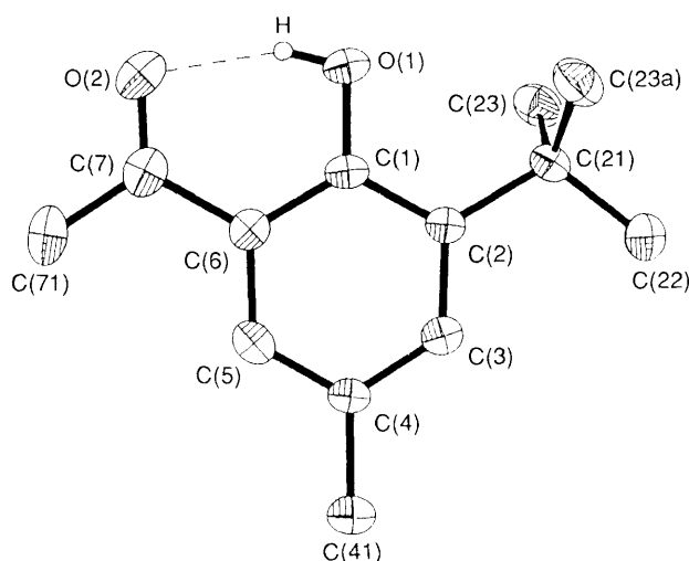
Fig. 2 The molecular structure of Hbhmpp 5 . Thermal ellipsoids are drawn at the 30% level. Only the hydrogen atom attached to O(1) is depicted; the remainder are omitted for clarity.
