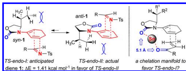
Scheme 3. Unexpected Switch in the Facial Preference
