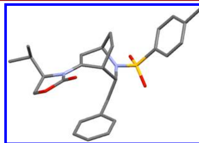
Figure 2. X-ray structure of endo-II cycloadduct 12b.
