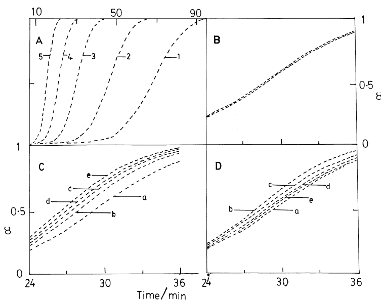
Fig. 1. Typical \alpha - t plots for the thermal decomposition of (A) pure \text{KIO}_4 at five temperatures ( 1.560 , 2.565 , 3.570 , 4.575 and 5.580 \text{ K} ), (B) \text{Cl}^- , (C) \text{SO}_4^{2-} and (D) \text{Ba}^{2+} doped \text{KIO}_4 at 570 \text{ K} . Dopant concentrations (mol%) — a: Nil; b: 10^{-4} ; c: 10^{-3} ; d: 10^{-2} ; e: 10^{-1} . In B curves a, b, c, d and e overlap in between the lines shown.
