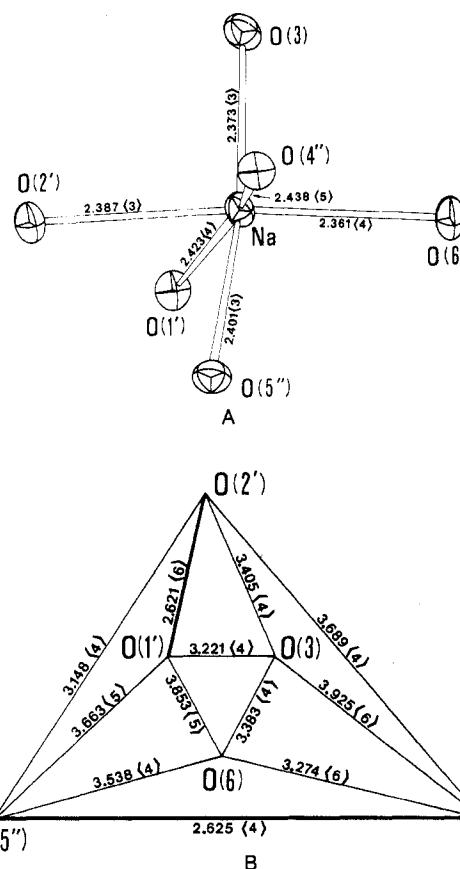
Figure 4. (A) An ORTEP drawing of sodium coordination polyhedron: single prime = -x, -y, 1-z ; double prime = -x, -y, -z . (B) A Schlegel projection of sodium coordination polyhedron.
