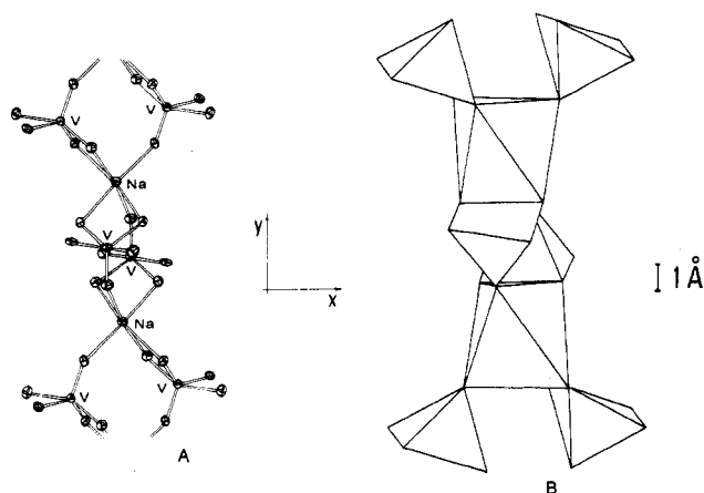
Figure 2. Two representations of the coordination polyhedra around vanadium and sodium along the chain of complex II, [(VO(salen))_2Na]^+ .
