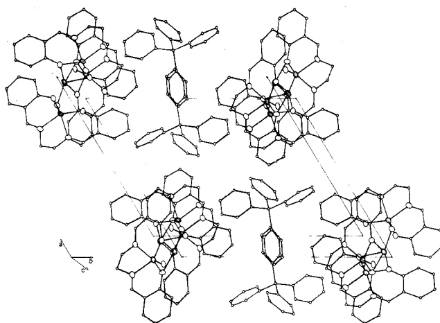
Figure 1. Crystal packing of [(VO(salen)) 2 Na]BPh 4 viewed nearly along the c direction.
