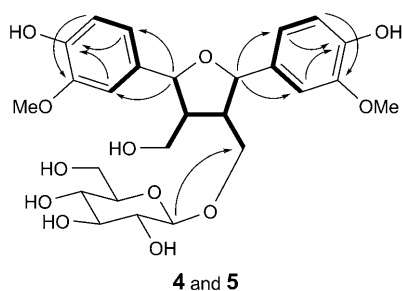
Fig. 4. ^1\text{H},^1\text{H} -COSY Correlations ( \Rightarrow ) and key HMBCs ( \text{H} \rightarrow \text{C} ) of 4 and 5
