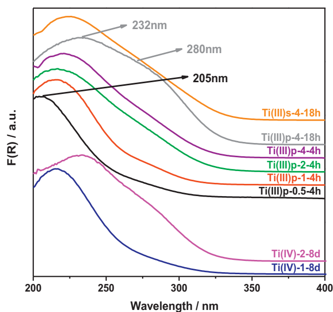
Fig. 2. UV region of the DRUV-visible spectra of the calcined samples Ti(III)APO-5 and Ti(IV)APO-5 with different titanium content.
