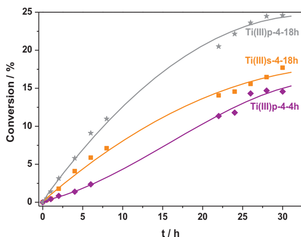
Fig. 4. Cyclohexene conversion over TAPO-5 catalysts prepared with different Ti(III) sources: Ti(III)s-4-18h (squares), prepared with aqueous hydrochloric acid solution of TiCl 3 , and Ti(III)p-4-4h (diamonds) and Ti(III)p-4-18h (stars) prepared with TiCl 3 powder.
