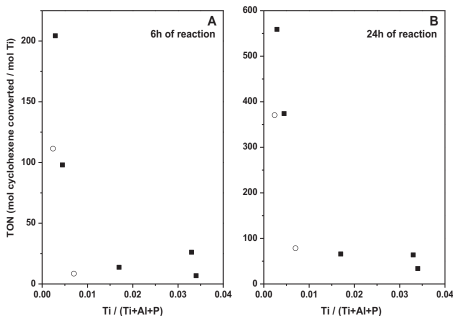
Fig. 6. Cyclohexene conversion per Ti center (TON) in Ti(III)APO-5 (full squares) and Ti(IV)APO-5 (open circles) samples with different titanium content after 6 h (A) and 24 h (B) of reaction.
