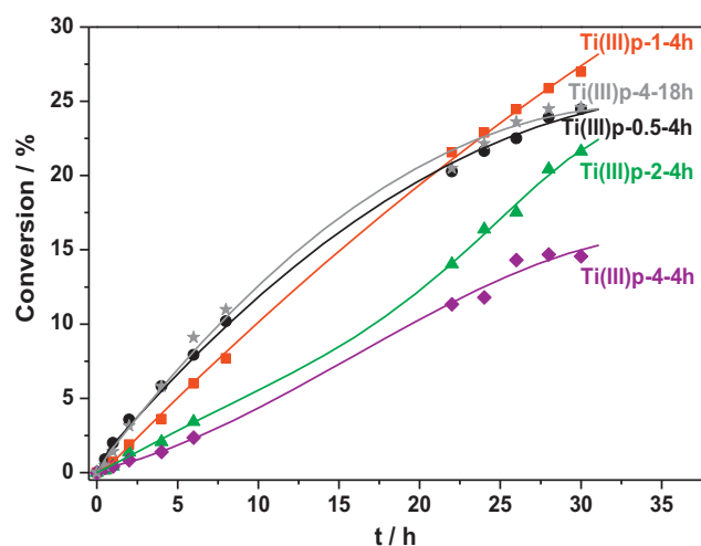
Fig. 5. Cyclohexene conversion over Ti(III)APO-5 catalysts prepared with \text{TiCl}_3 powder and different titanium content: Ti(III)p-0.5-4h (circles), Ti(III)p-1-4h (squares), Ti(III)p-2-4h (triangles), Ti(III)p-4-4h (diamonds) and Ti(III)p-4-18h (stars).
