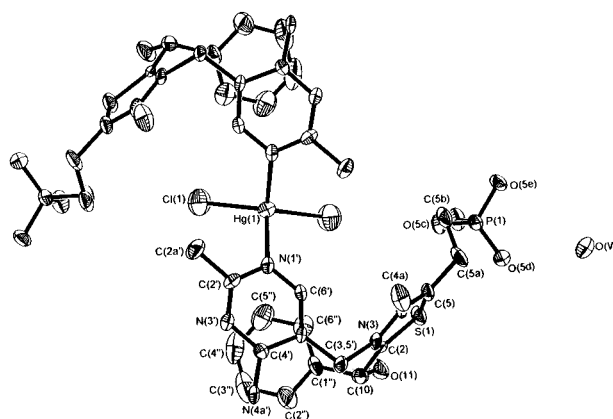
Figure 2. Crystal structure of HgL 2 Cl 2 .
