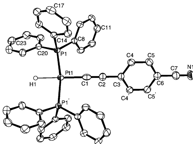
Figure 1. ORTEP view of [\text{trans}\text{-PtH}\{\text{C}\equiv\text{C}(4\text{-CN})\text{C}_6\text{H}_4\}(\text{PPh}_3)_2] ( 1b ). Ellipsoids are drawn at the 50% probability level. Aromatic hydrogen atoms have been omitted for clarity.
