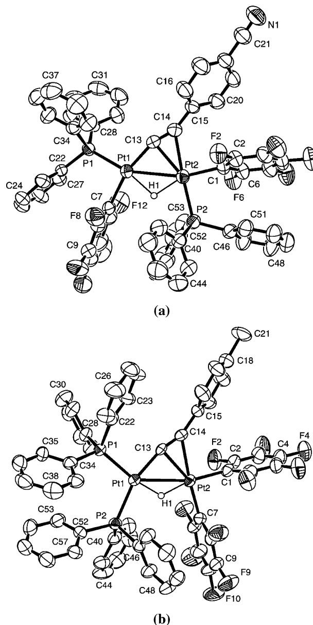
Figure 2. Molecular structures of (a) [ trans -(PPh 3 )(C 6 F 5 )Pt(μ-H){μ-1κC σ :η 2 -C≡C(4-CN)C 6 H 4 }Pt(C 6 F 5 )(PPh 3 )] ( 3b ) and (b) [ cis,cis -(PPh 3 ) 2 Pt(μ-H){μ-1κC σ :η 2 -C≡C(4-CH 3 )C 6 H 4 }Pt(C 6 F 5 ) 2 ] ( 4a ). Ellipsoids are drawn at the 50% probability level. Hydrogen atoms have been omitted for clarity.
