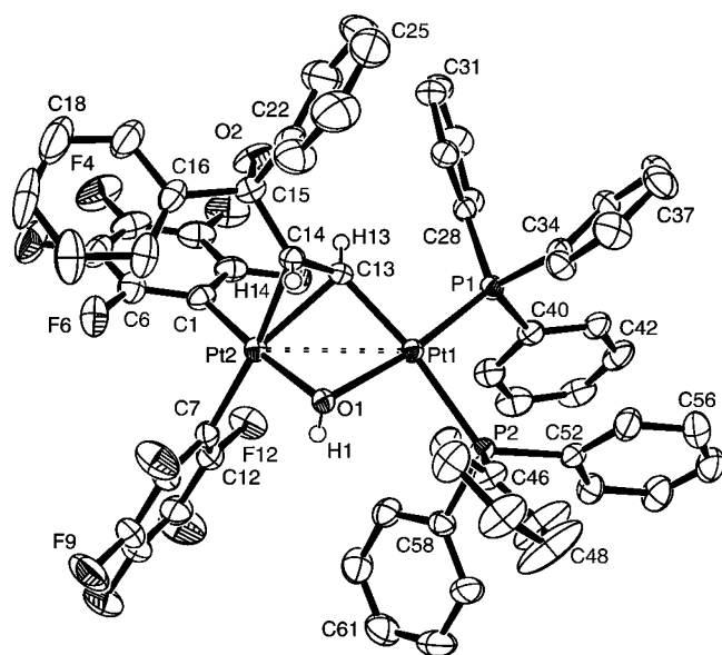
Figure 5. ORTEP view of [cis,cis\text{-}(\text{PPh}_3)_2\text{Pt}\{\mu\text{-}1\kappa\text{C}^\alpha\text{-}\eta^2\text{-CH}=\text{CHC}(\text{OH})\text{Ph}_2\}(\mu\text{-OH})\text{Pt}(\text{C}_6\text{F}_5)_2] ( 5f ). Ellipsoids are drawn at the 50% probability level. Aromatic hydrogen atoms have been omitted for clarity.
