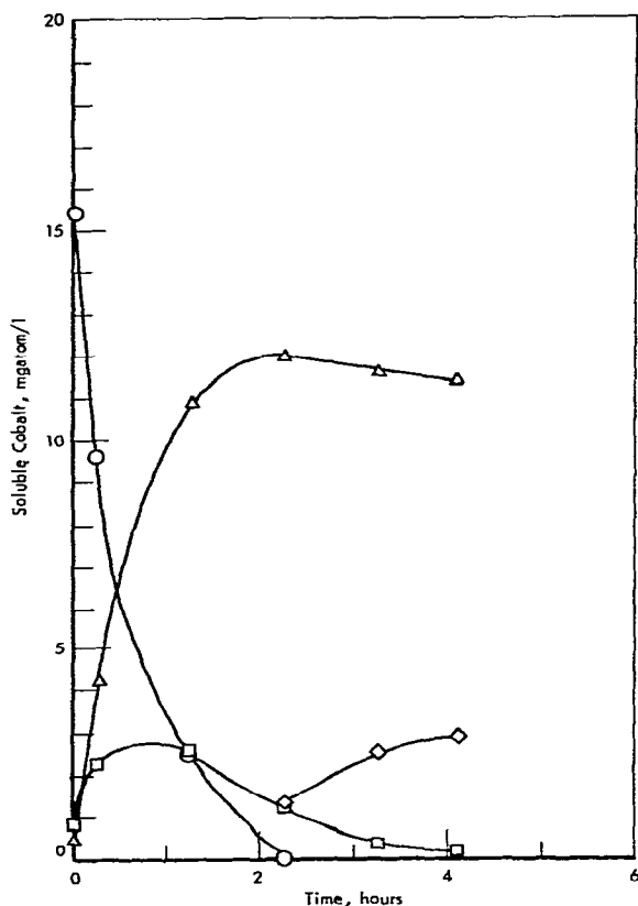
Fig. 1. Conversion of \pi -C 4 H 7 Co(CO) 2 PBU 3 (I) under synthesis gas, 110 \pm 2^\circ , 500 psig, H 2 /CO = 1.5 in 1-heptene. From data of samples reduced to atmospheric conditions. O \pi -C 4 H 7 Co(CO) 2 PBU 3 (I); \Delta \text{Bu}_3\text{PCo(CO)}_3\text{-Co(CO)}_3\text{PBU}_3 (II); \square \pi -C 4 H 7 Co(CO) 3 (III); \diamond \text{Bu}_3\text{PCo(CO)}_3\text{-Co(CO)}_4 (IV).
