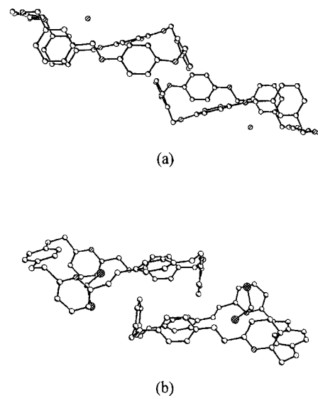
Figure 3. Packing in the crystal lattice inclusion complex of M2 with water (a) and molecular inclusion complex of M2 with dichloromethane (b) (hydrogen atoms are omitted for clarity).
