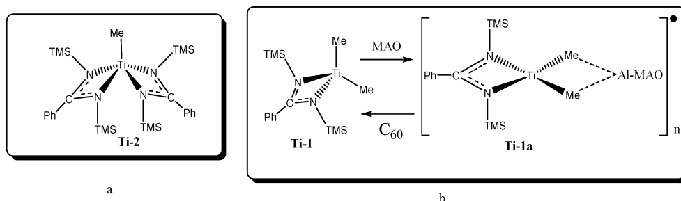
Scheme 4. Proposed Ti(III) Intermediates in the Activation of Complexes 1 and 2 with MAO
