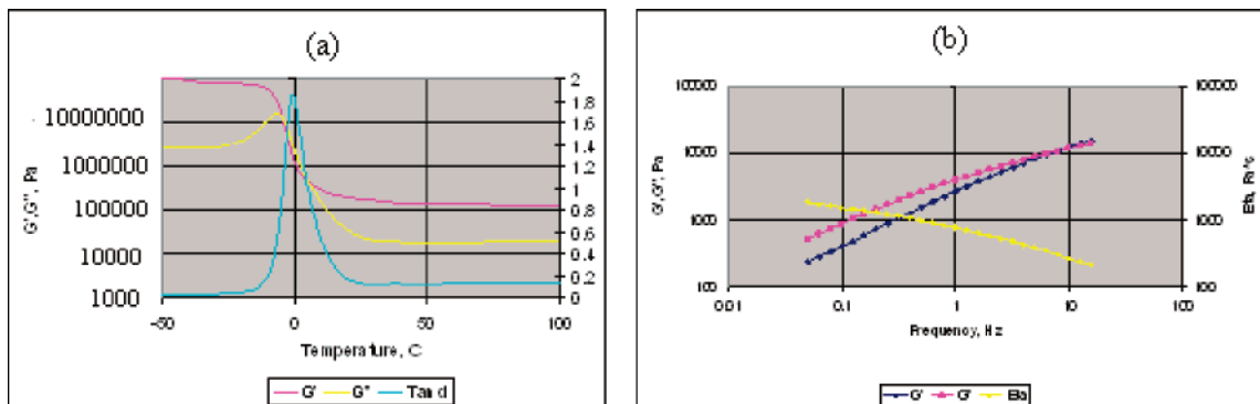
Figure 10. DMTA thermogram for the polypropylene PP-1 (a) and frequency dependences of the storage and loss moduli, and of the complex viscosity for the blend of polymer PP-1 measured at 180 ^{\circ}\text{C} (b).
