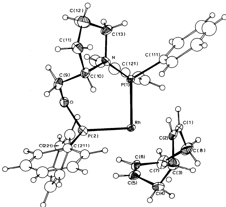
Fig. 1. A view of the cation [\text{Rh}(\text{COD})((S)\text{-Prolophos})]^+ .
