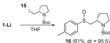
Scheme 2. Alkylation of Lithium p -toluenesulfonate ( 1-Li ) with L-Prolinyl Iodide ( 15 )
