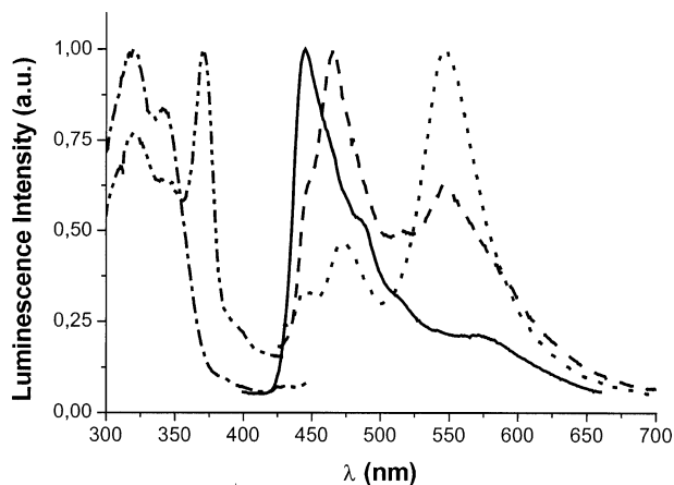
Figure 8. Excitation and emission spectra of [(\text{C}_6\text{F}_5)_4\text{PtCd}(\text{cyclen})] ( 1 ) in \text{CH}_2\text{Cl}_2 solution (77 K). Excitation: (·····) \lambda_{\text{em}} 525; (---) \lambda_{\text{em}} 466. Emission: (—) \lambda_{\text{ex}} 340; (---) \lambda_{\text{ex}} 360; (— · —) \lambda_{\text{ex}} 370.
