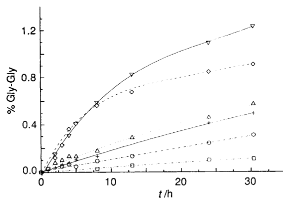
Fig. 1 Diglycine formation in the system 1.0 \text{ mol dm}^{-3} glycine, 0.5 \text{ mol dm}^{-3} \text{ CuCl}_2 and 3 \text{ mol dm}^{-3} \text{ NaCl} at different pH and 80 °C. pH 1.93 (◇), 2.18 (▽), 2.52 (△), 2.60 (+), 2.74 (○) and 3.04 (□)
