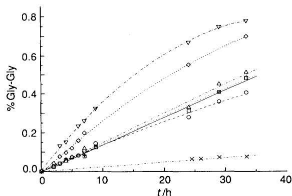
Fig. 5 Rate of peptide formation at 80 °C in the system 1.0 mol dm -3 glycine, 0.5 mol dm -3 CuCl 2 and 1.5 mol dm -3 MCl 2 or 3.0 mol dm -3 MCl for all cations: NH 4 + (□), Na + (+), K + (○), Cs + (×), Mg 2+ (▽), Ca 2+ (◇) and Ba 2+ (△)
