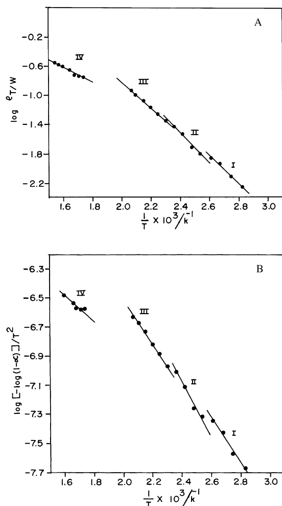
Fig. 5. (a) Plot of \log \rho_T/w vs 1/T \times 10^3 K^{-1} of complex I. (b) Plot of \log [-\log(1-\alpha)]/T^2 vs 1/T \times 10^3 K^{-1} of complex I.
