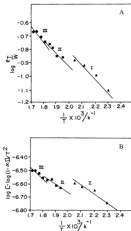
Fig. 6. (a) Plot of \log \rho_T/w vs 1/T \times 10^3 K^{-1} of complex II. (b) Plot of \log [-\log(1-\alpha)]/T^2 vs 1/T \times 10^3 K^{-1} of complex II.
