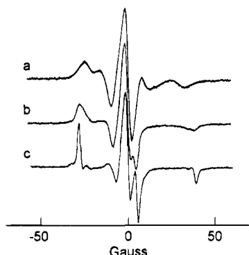
Figure 1. EPR spectra of (a) [5'-d(GCC TAC ATG QGA CG)-5'-d(CGT CPC ATG TAG GC)] (20 °C) overlaid with a simulated spectrum (see below); (b) [5'-d(GCC TAC ATG T*GA CG)-5'-d(CGT CAC ATG TAG GC)] (0 °C) in 50% w/v sucrose, where T* is in the spin probe as in 1; (c) [5'-d(GCC TAC ATG QGA CG)-5'-d(CGT CPC ATG TAG GC)] (0 °C) in 50% w/v sucrose. Samples contained 10 mM phosphate buffer (pH 7.0), 115 mM Na + , and 0.1 mM EDTA. A least-squares fit of the spectrum c following 1 G Lorentzian convolution yielded the following tensor values: A_{xx} = 6.68 G, A_{yy} = 5.41 G, A_{zz} = 33.9 G, g_{xx} = 2.0076 , g_{yy} = 2.0061 , g_{zz} = 2.0028 ( \chi^2 = 1.7 ). 13 The tensors were used to simulate spectrum a, yielding a single correlation time of 7.6 ns ( \chi^2 = 3.2 ) assuming an isotropic model.
