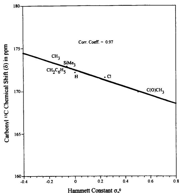
Fig. 2. Correlation of ^{13}\text{C} NMR carbonyl chemical shift data with \sigma_p^0 .
