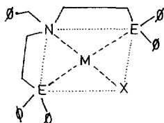
Scheme 1. M = Rh(I), X = CO; M = Ir(I), Pd(II); X = Cl, \text{SnCl}_3 ; E = P, As.
