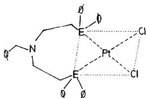
Scheme 2. \text{E} = \text{P}, \text{As} .
