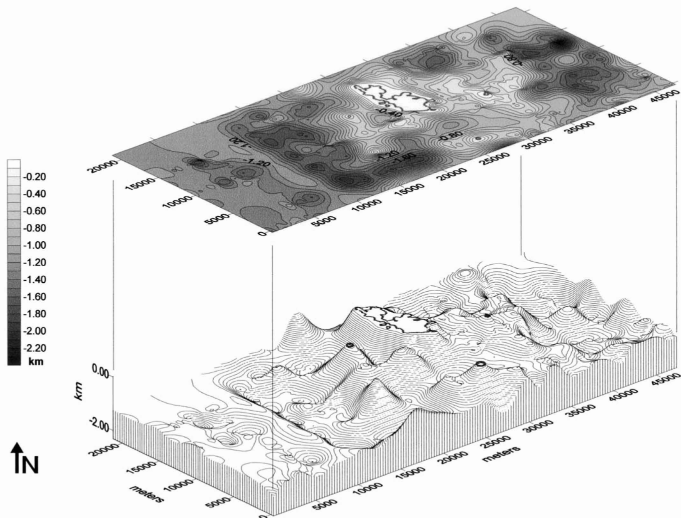
FIG. 7. Bi- and tridimensional view of bedrock topography in the Frontier Mountain area.
