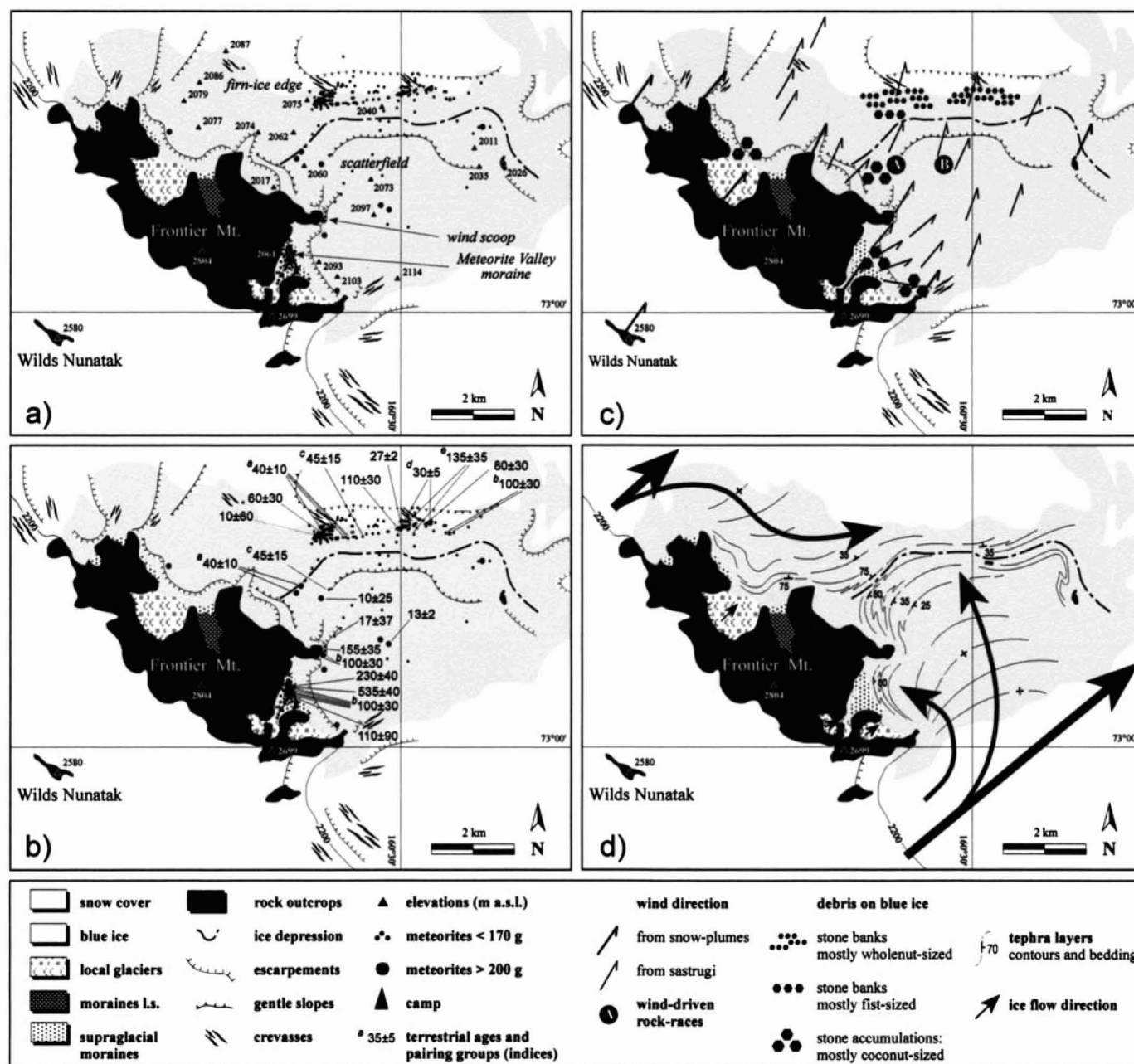
FIG. 3. Sketch maps of the Frontier Mountain blue ice field. (a) Main geomorphological data and meteorite distribution. (b) Geographic distribution of terrestrial ages of meteorites and pairing groups available from literature ( i.e. , Wieler et al. , 1995; Terribilini et al. , 2000; Welten et al. , 2001; Welten, 2001, pers. comm.); indices (a) and (b) correspond to the FRO 90001 and FRO 90174 showers recognized by Welten et al. (2001) and Welten (2001, pers. comm.), respectively; other indices indicate possible pairs according to Welten et al. (2001) and Welten (2001, pers. comm.). (c) Wind field, geographic distribution of local stones and location of the wind-driven rock-races. (d) Generalized contours and bedding of tephra layers and ice flow pattern.
