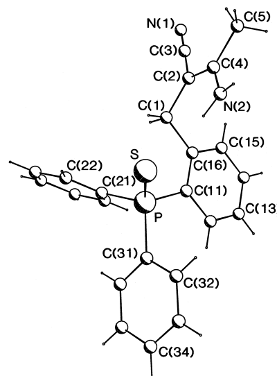
Fig. 1. The structure of one of the independent molecules of the enamine 7. The labelling scheme for each molecule is generated by adding 1 or 2 appropriately; for example N(1) becomes N(11) for molecule 1 and N(21) for molecule 2.
