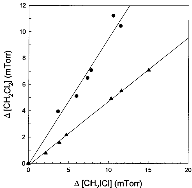
Figure 8. Yield of CH 2 Cl 2 versus loss of CH 2 ICl following irradiation of CH 2 ICl/Cl 2 /N 2 (●) and CH 2 ICl/Cl 2 /O 2 /N 2 (▲) mixtures at a total pressure of 100 Torr; see text for details.
