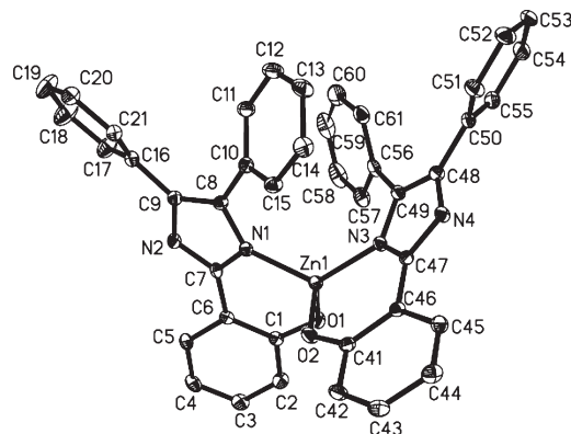
Figure 7. Molecular structure of Z2 ·3CH 3 OH with thermal ellipsoids drawn at the 50% probability level. Some hydrogen atoms and three methanol solvent molecules have been omitted for clarity.
