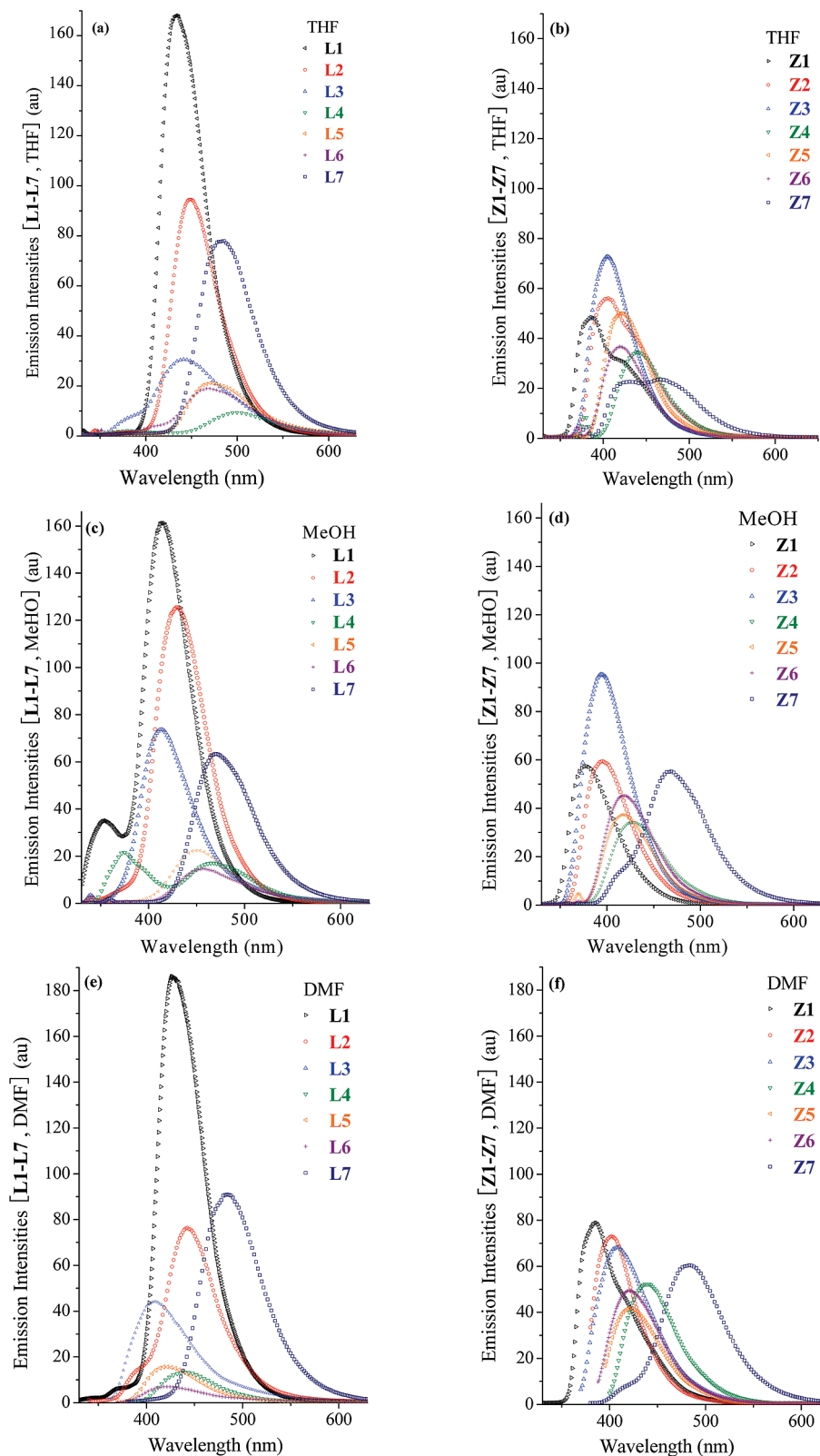
Figure 9. Relative emission intensities of ligands L1–L7 and their corresponding complexes Z1–Z7 in THF (a and b), MeOH (c and d), and DMF (e and f) solutions, respectively.
