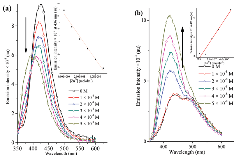
Figure 13. Fluorescence response on \text{Zn}^{2+} titration ( 0 – 5 \times 10^{-8} M) for L2 (a) and L4 (b).
