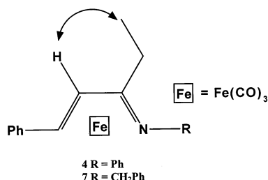
Fig. 2. Complexes 4 and 7.
