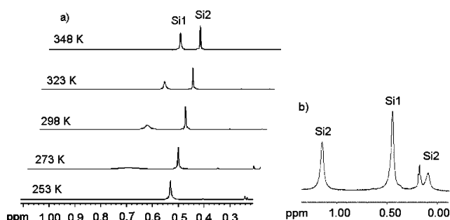
Figure 6. (a) Variable-temperature ^1\text{H} NMR spectra ( \text{C}_7\text{D}_8 ) of 4 . Broadening of the \text{SiMe}_3 protons as the temperature is lowered. At 348 K two peaks are observed for the \text{SiMe}_3 protons labeled Si(1) and Si(2). When the sample is cooled, the protons for Si(1) broaden into the baseline. (b) ^1\text{H} NMR spectrum ( \text{C}_7\text{D}_8 ) of 4 at the low-temperature limit (188 K). Below the coalescence temperature, two peaks are observed for the Si(1) protons at 1.13 and 0.09 ppm in a 5:1 ratio.
