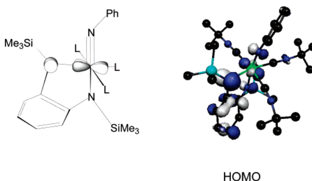
Figure 3. Interaction of diamide lone pairs and isocyanide ligand with metal d xy orbitals. (Orbitals are displayed at the 0.05 au isocontour level.)
