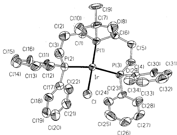
Fig. 1. Structure of [^1\text{BuP}(\text{CH}_2\text{CH}_2\text{CH}_2\text{PPh}_2)_2]\text{IrCl} ; selected bond lengths (Å) and angles (deg): Ir–Cl, 2.404(6); Ir–P(1), 2.212(6); Ir–P(2), 2.280(7); Ir–P(3), 2.288(6); Cl–Ir–P(1), 166.4(2); Cl–Ir–P(2), 88.0(2); Cl–Ir–P(3), 88.8(2); P(1)–Ir–P(2), 94.0(2); P(1)–Ir–P(3), 94.8(2); P(2)–Ir–P(3), 155.3(2).
