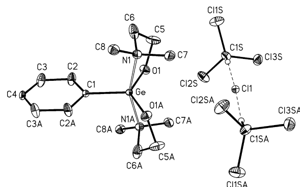
Figure 1. Crystal structure of 1b ·2CHCl 3 with 40% probability ellipsoids (most H atoms are omitted for clarity). The label A denotes symmetrically equivalent atom relative to the 2-fold axis. The coordination Ge–N bonds are shown by double lines and the H-bonds are shown by dashed lines. Selected bond lengths (Å) and angles (deg): Ge–O1 1.780(3), Ge–C1 1.912(4), Ge–N1 2.092(4), Ge···Cl1 4.668(2), O1–Ge–C1 113.8(2), O1–Ge–N1 85.3(2), N1–Ge–C1 101.1(1), O1–Ge–O1 i 132.5(3), N1–Ge–N1 i 157.8(2), O1–Ge–N1 i 85.8(2). Symmetry operation i: 1 – x, y, 1.5 – z.
