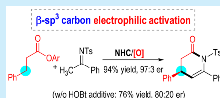
Scheme 1. NHC-Catalyzed \beta -sp 3 Carbon Functionalization of Saturated Esters
