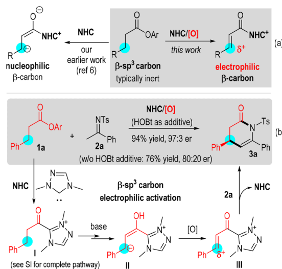
Scheme 1. NHC-Catalyzed \beta -sp 3 Carbon Functionalization of Saturated Esters
