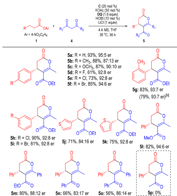
Scheme 3. Examples of Substituted Ketones a
